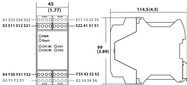
Figure 6 - Dimensions [mm (in.)]
