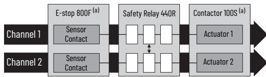
Figure 7 - Safety Circuit
