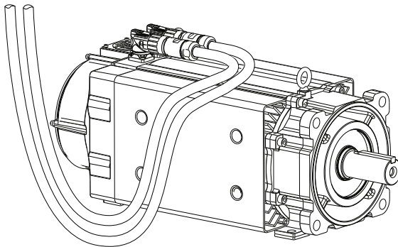
Drip loop for foot mounted motor with connectors on top.
