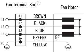
VPC-FAN300 Terminal Box Wiring
