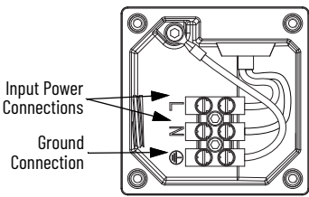
VPC-B165xx Motors
